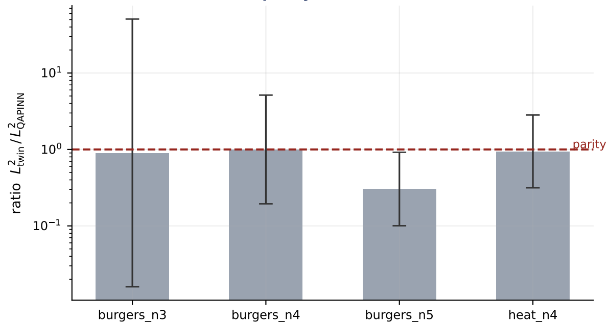
(b) Paired ratio with 95% CI (above parity \Rightarrow QAPINN better)
